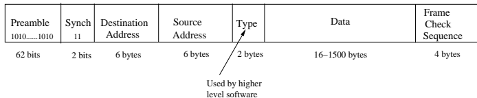
Ethernet Packet Format
